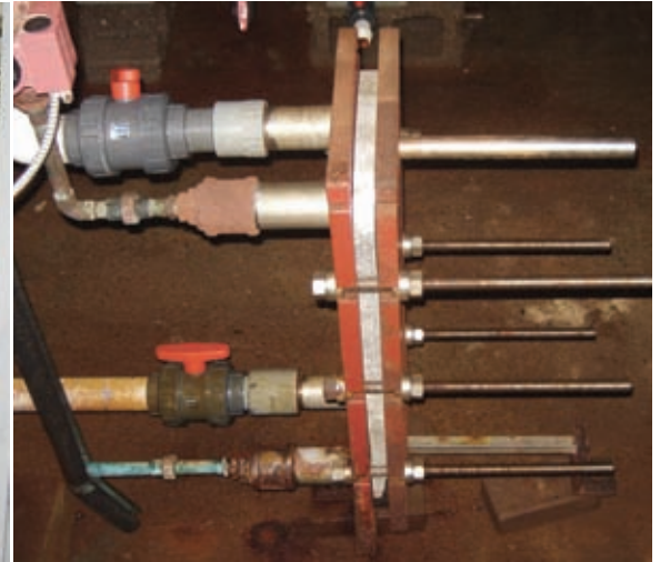
Properly sized water-to-water heat exchangers should perform at greater than 90% efficiency.
